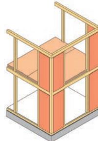
Traditional wooden frame construction + CLT
